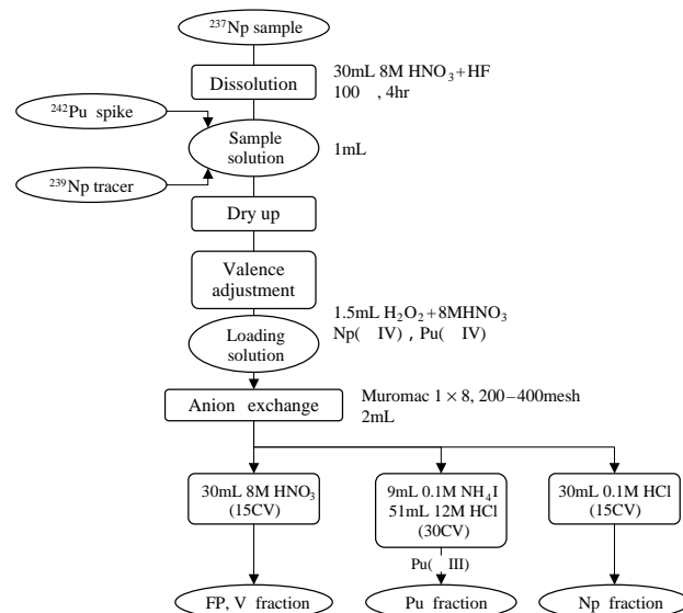
Figure 3. Flow sheet for chemical separation of irradiated ^{237}\text{Np} sample.
