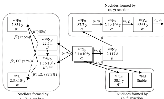
Figure 1. Nuclear reaction chain started from ^{237}\text{Np} .
