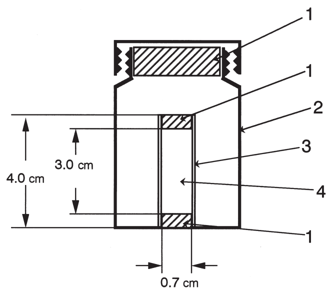
Figure 1. Schematic diagram of the ^{222}\text{Rn} sample and the counting vial for measuring the counting efficiency of the air luminescence method: 1. silicone rubber stopper; 2. counting vial; 3. quartz tube; 4. ^{222}\text{Rn} sample.
