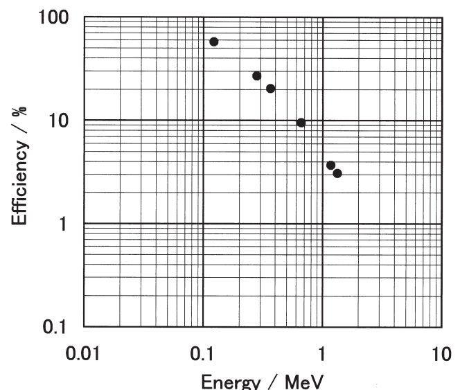
Figure 3. Full energy peak efficiencies as a function of \gamma -ray energy.
