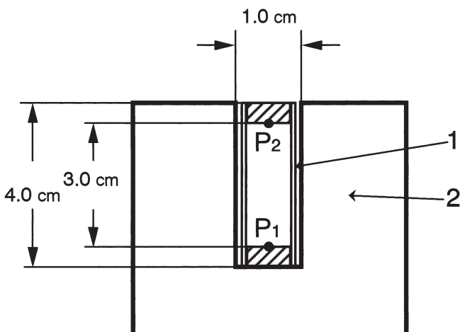
Figure 2. The position of the EGP type point source in the well of Ge detector for the determination of the full energy peak efficiency: 1. quartz tube; 2. Ge well detector; P_1 , the position on the center line of the well at 0.5 cm from the lower end of the tube; P_2 , the position on the center line of the well at 0.5 cm from the upper end of the tube.
