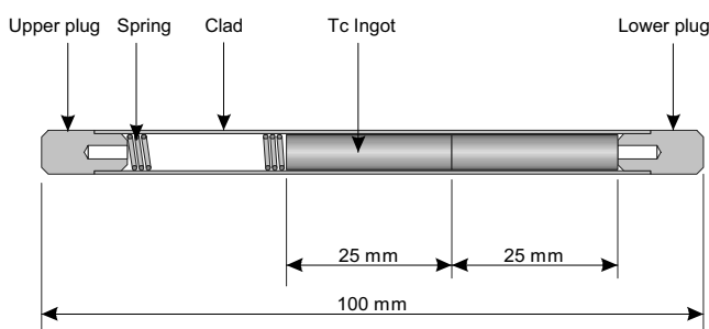
Figure 1. ANTICORP 1 pin drawings.
