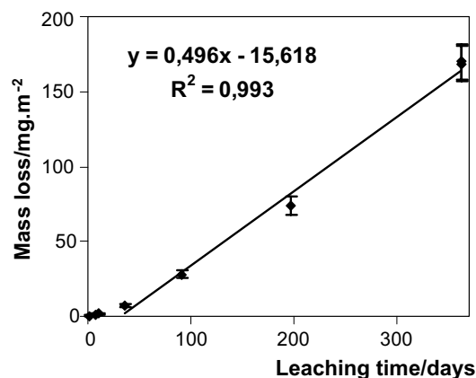
Figure 6. Mean alteration rate of Tc metal in pure water at 25 °C.
