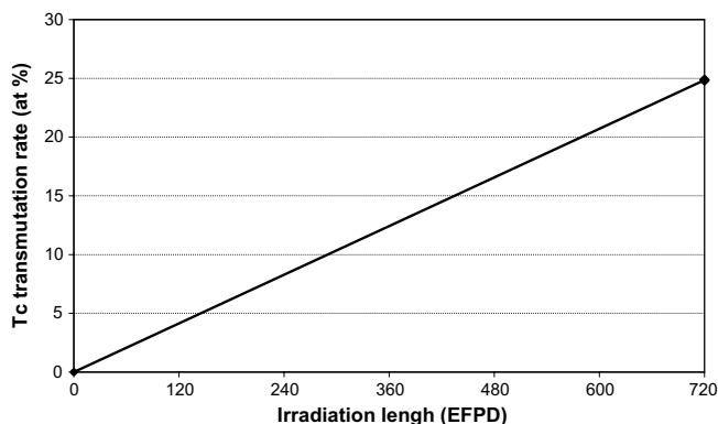
Figure 5. Evolution of the ^{99}\text{Tc} transmutation rate during irradiation in the front pin.
