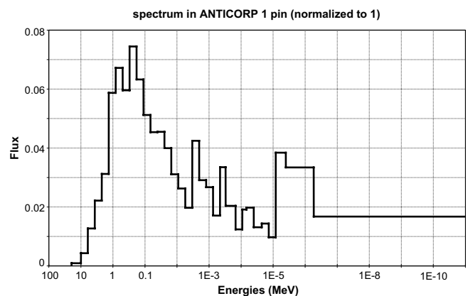
Figure 4. Spectrum (33 groups) in ANTICORP 1 irradiation.
