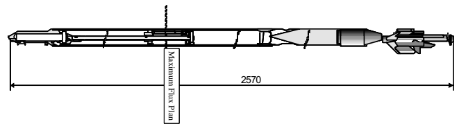
Figure 3. Irradiation capsule.
